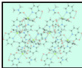
Fig. 3. A packing diagram of compound (I) viewed down the a axis.
