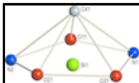
Fig. 2. The coordination polyhedron of the \text{Bi}^{\text{III}} ion in compound (I).
